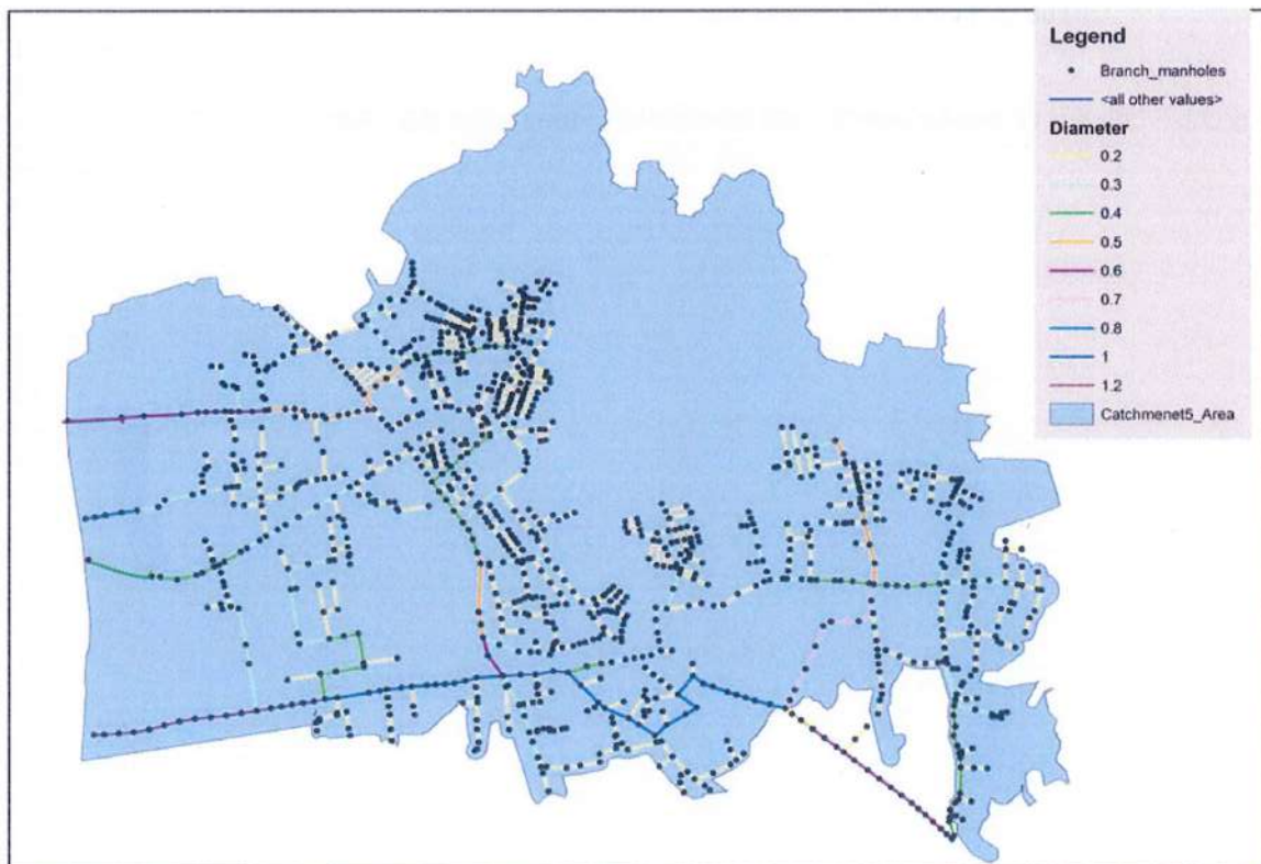
Figure 4: Preliminary design of sewerage network
